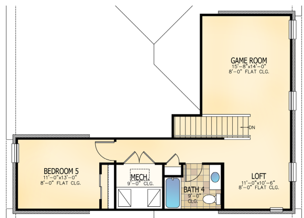
Opt. Game Rm/Bath 4 & Bed 5
