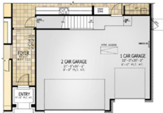
Partial Main Floor Plan - Opt Texas Basement
