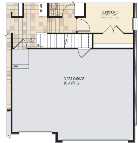
Partial Main Floor Plan w/ Opt. Game room or w/ Opt. Game Room w/ Bedroom
