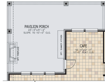
Opt. Pavilion Porch
