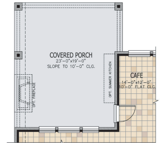
Opt. Ext. Covered Porch
