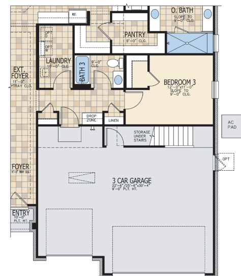
Partial Main Floor At Opt. Texas Basement
