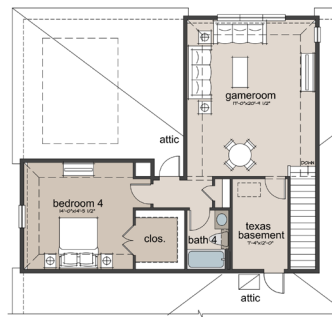
optional texas basement with game room and bedroom 4 - upper floor
